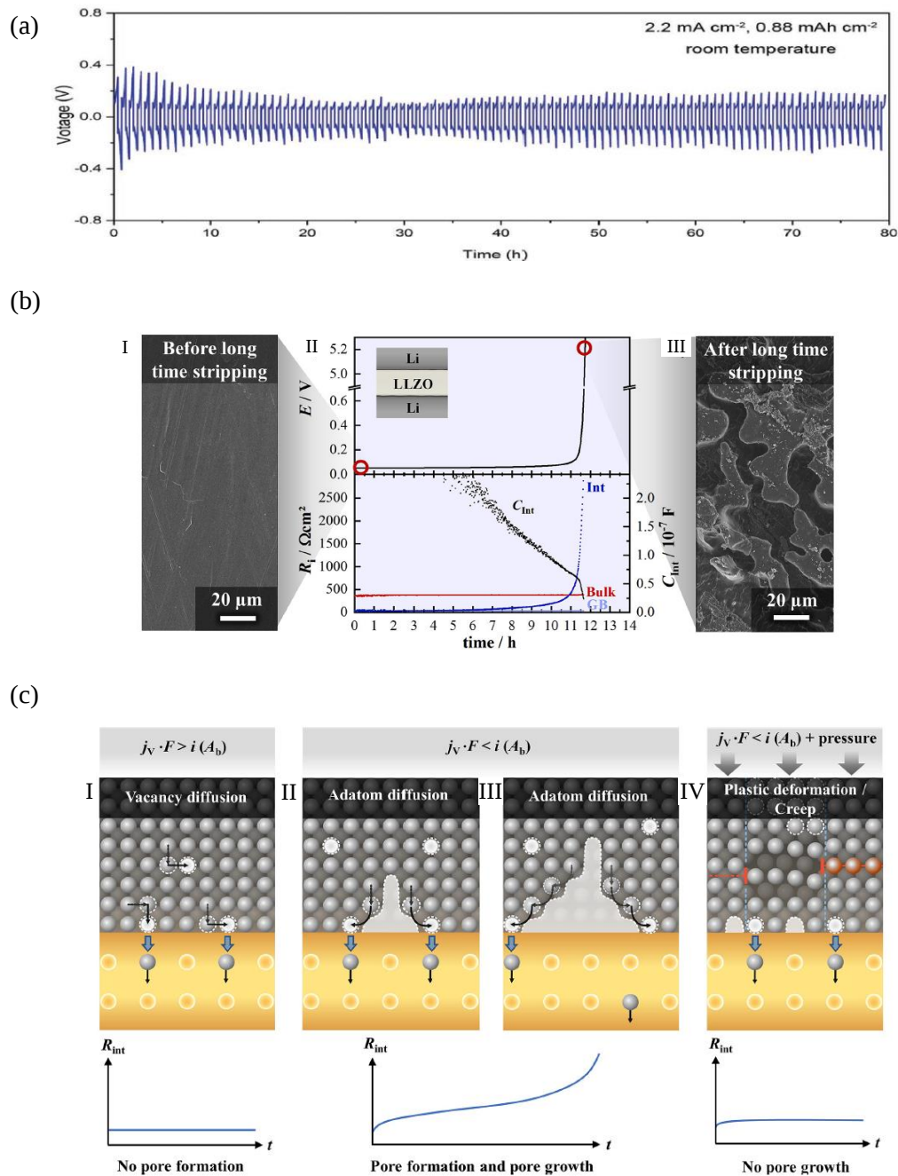
Figure 6. The development of negative electrode for CLBs. (a) Galvanostatic cycling of Li/LLZO/Li at 2.2 \text{ mA cm}^{-2} for 0.88 \text{ mA h cm}^{-2} for 100 cycles. 77 Reproduced with permission. 77 Copyright 2019, Wiley-VCH. (b) Morphology of the lithium metal electrode before assembling the symmetric cell (I) and after stripping at 100 \text{ } \mu\text{A cm}^{-2} anodic load (III). The potential profile and impedance contributions shows a complete contact loss of Li electrode after around 12 h of stripping (II). (c) Schematic of the different mechanisms that facilitate charge transfer at the lithium metal electrode under anodic load (limiting cases). 98 (I) local current density does not exceed the vacancy diffusion limit. (II, III) local current density exceeds the diffusion limit (IV) external pressure is applied. 98 Reproduced with permission. 98 Copyright 2019, American Chemical Society.
